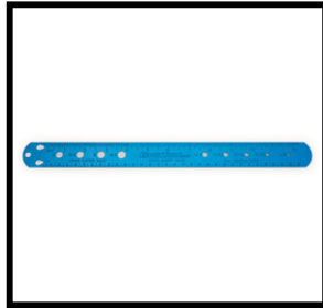
SBC-1 Spoke, Bearing, and Cotter Gauge
